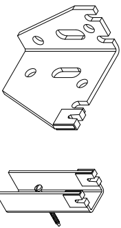
LN Type Bracket
